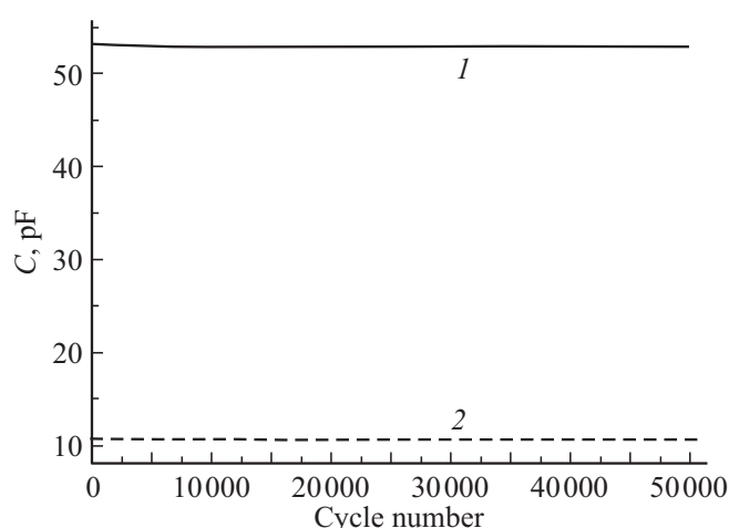
Figure 6. Maximum and minimum capacitance values of Si/HfO 2(ann) /Ni structures depending on switching cycles. Numbers of curves: 1 (solid line) — measurements at a voltage of +3.5 V, 2 (dashed line) — measurements at a voltage of -3.5 V.
