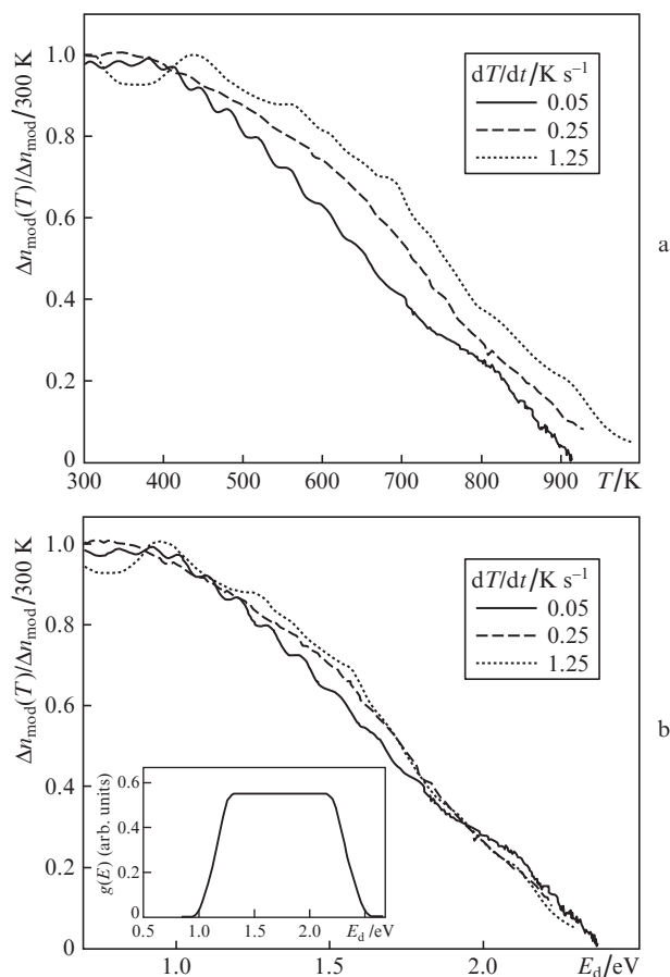
Figure 3. (a) Annealing dependences of the normalised value \Delta n_{\text{mod}} of FBG, measured at three heating rates and written to the pristine fibre. (b) Similar dependences in the coordinates of demarcation energy E_d in the case of the best superposition.
