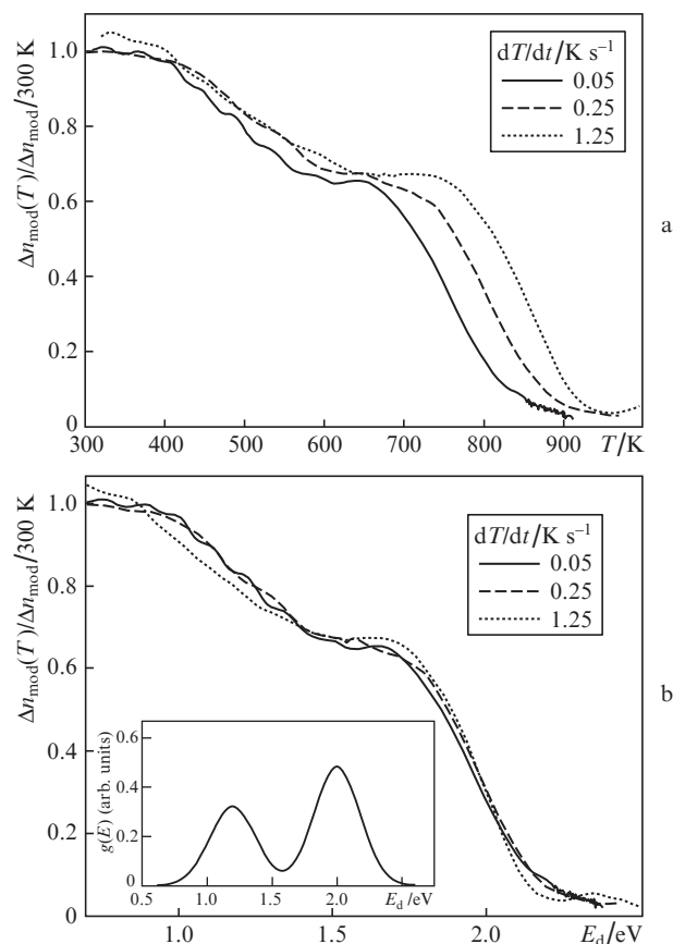
Figure 4. (a) Annealing dependences of a normalised value \Delta n_{\text{mod}} of FBG, measured at three heating rates and written in the \text{H}_2 -loaded fibre. (b) Similar dependences in the coordinates of demarcation energy E_d in the case of the best superposition.
