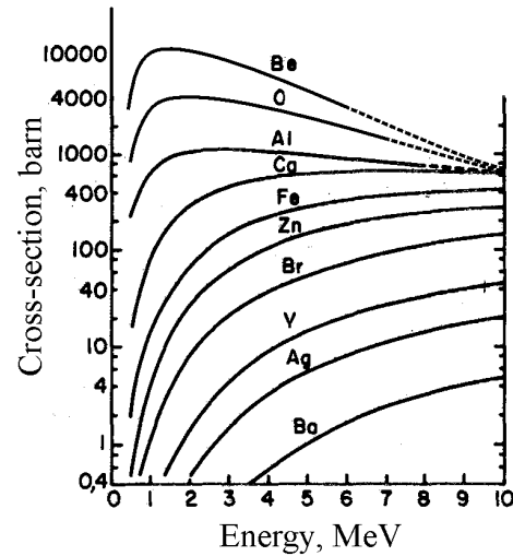
Figure 2. Energy dependences of the cross-section excitation for K_{\alpha} different elements lines yield in conditions of H^+ ion beam using of the exciting agent [4].
