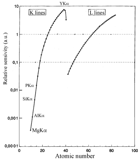
Figure 1. Cross-sections excitation for K_{\alpha} and K_{\beta} different elements lines yields in conditions of MoK_{\alpha} radiation flux using as the exciting agent [1].
