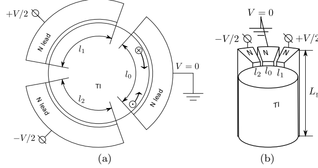
FIG. 1: (a) Helical edge state of 2D TI coupled to the leads (b) Helical surface state of 3D TI coupled to the leads
