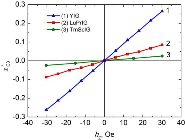
Fig. 2. Measured dependence of \chi'_{C3} versus magnetic field h_z , applied normal to the film plane for different garnet.
