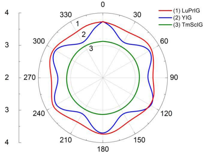
Fig. 1. Experimental angular dependence of transverse susceptibility \chi'(\varphi) in a rotating field H = 4 mT in plane (111) for some iron garnets.
