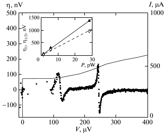
Fig. 7. Current–voltage characteristic of heterojunctions (solid curve) and detector response to electromagnetic radiation of frequency 119.5 GHz (dots). The inset shows the dependences of the main response for V_1 = 246 \mu\text{V} on the microwave power (triangles) and fractional response for V_{1/2} = 123 \mu\text{V} (rhombs).
