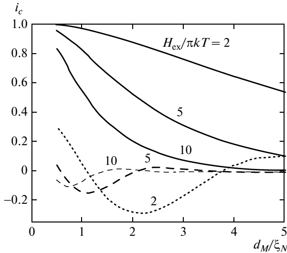
Fig. 6. Theoretical dependences of normalized critical current i_c on normalized thickness d_M/\xi_N of the M interlayer for three values of normalized exchange field H_{ex}/\pi kT . Solid curves correspond to the AF interlayer, while dashed curves correspond to the F interlayer.
