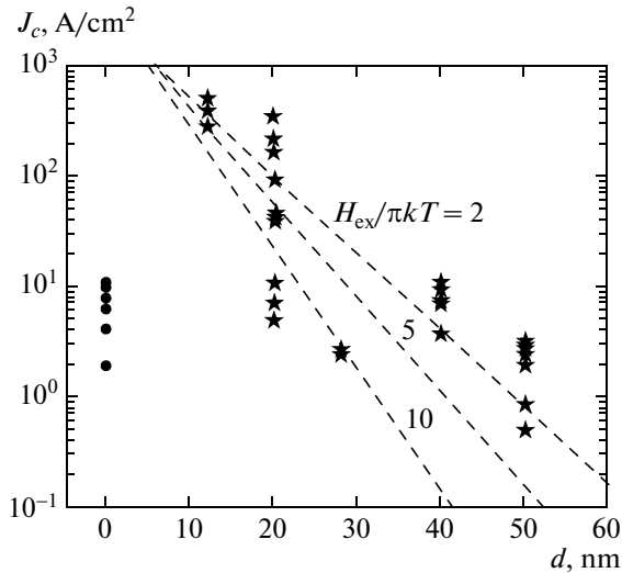
Fig. 5. Experimental results on the dependence of the superconducting current density on d_M for heterostructures with a CSCO interlayer with doping level of x = 0.5 (★) and for heterostructures without the M interlayer (●). Dashed lines show the theoretical dependences of the critical current on the thickness of the AF interlayer for three values of normalized exchange field H_{\text{ex}}/\pi kT = 2, 5, and 10 . Theoretical dependences are the normalized critical current density choosing interlayer thickness in accordance with the condition of best matching of the theory to experiment ( \xi_{\text{AF}} = 10 nm).
