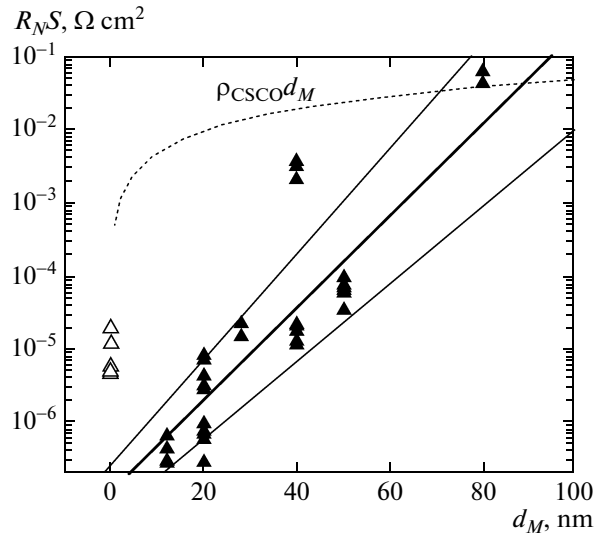
Fig. 4. Dependence of characteristic resistance R_N S of heterojunctions on interlayer thickness d_M (▲). Resistance of heterojunctions without M interlayer (△). The bold line shows the exponential dependence R_N S(d_M) with a characteristic growth length of 6 \pm 1 nm, obtained from statistical processing of experimental data. Fine lines show the error in determining the characteristic length. The dotted curve is the product of resistivity \rho_{CSCO} of the M interlayer, which was determined from measurements on an autonomous film, by thickness d_M .
