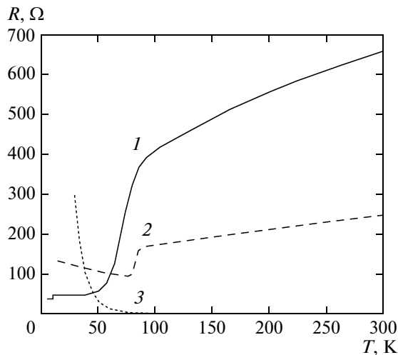
Fig. 3. Temperature dependence of resistance: 1—no. 612 sample, d_M = 20 nm, L^2 = 10 \times 10 \mu\text{m}^2 ; 2—no. 610 sample, d_M = 40 nm, L^2 = 50 \times 50 \mu\text{m}^2 ; 3— \rho d_M/L^2 ( \rho is the resistivity) for an autonomous \text{Ca}_{0.5}\text{Sr}_{0.5}\text{CuO}_2 film deposited on the NGO substrate, d_M = 40 nm, L^2 = 50 \times 50 \mu\text{m}^2 .
