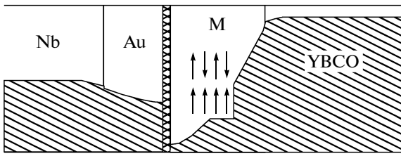
Fig. 1. Schematic representation of variation in the condensate wavefunction for heterostructures under investigation. The current is set along the c (horizontal) axis of the structure. The bold line shows the interface between the Au film and the M interlayer that makes the main contribution to the resistance of the structure. In the theoretical analysis, the M interlayer is represented as a multilayer structure with collinear directions of magnetization in the layers.
