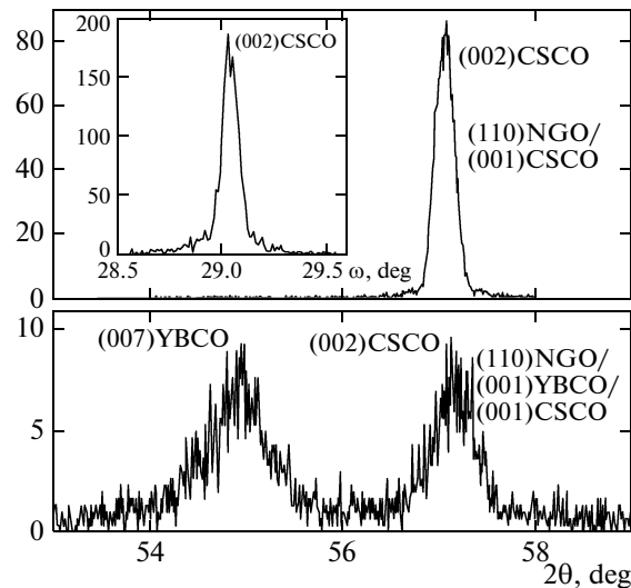
Fig. 2. X-ray 2\theta-\omega spectra and rocking curves ( \omega scan) of CSCO films ( x = 0.15 ) with a thickness of d_M = 50 nm deposited on NGO substrates (top). The 2\theta-\omega spectrum for the CSCO/YBCO/NGO heterostructure ( d_M = 100 nm) (bottom).
