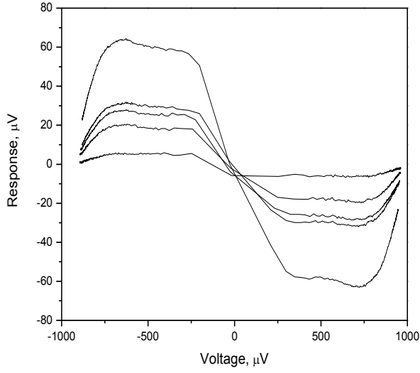
Fig. 5. Voltage response at lower levels of signal in the range 1-4 K. Standard bolometric response observed at about half-gap voltage bias, and at lower bias around quarter gap voltage corresponding to higher nonlinearity appears a direct detector response.
