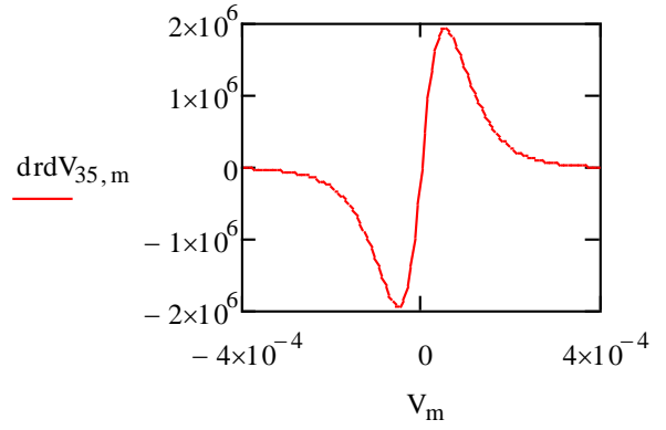
Fig. 7. Second derivative of normalized IV curve at 350 mK.
